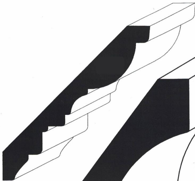
AWP-1420 3/4" x 4-5/8"
